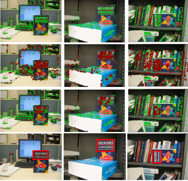
Fig. 2. Pattern discovery result. (1) 1st row: SIFT extraction results, each green point represents a visual primitive p \in \mathcal{D} ( |\mathcal{D}| = 3,084 ). (2) 2nd row: visual primitive pruning results based on individual SIFT matching. Red points are valid visual primitives p \in \mathcal{D}^1 ( |\mathcal{D}^1| = 1,078 ) and green points are those pruned. (3) 3rd row: pattern discovery based on fast spatial neighborhood matching with neighborhood size K = 25 and matching threshold \lambda = 10 . Red points are discovered visual primitives p \in \mathcal{D}^K ( |\mathcal{D}^K| = 316 ) that belong to the common spatial pattern. (4) 4th row: discovered spatial common pattern by fusing the discovered visual primitives.
